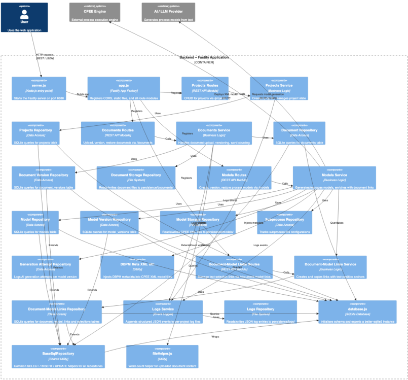
Figure 4 Backend Component
